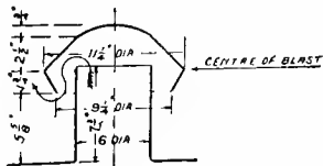
Fig. 4305. THE TORNADO CANOPY.
